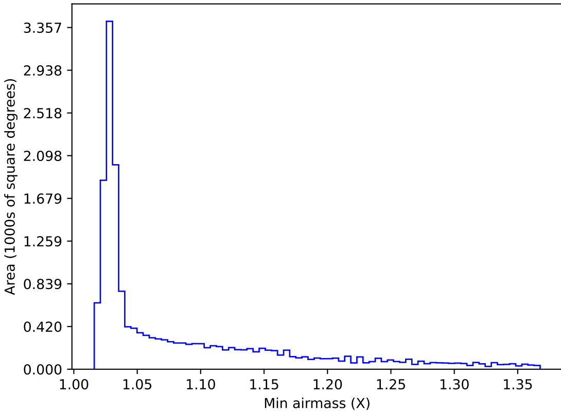
too_elab_r16_d2_giz_v3.4_10yrs WFD i band: Min airmass
