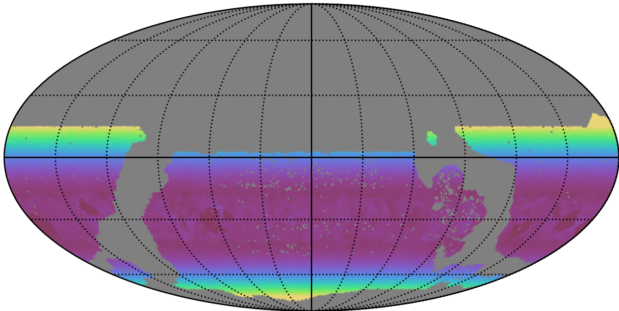
too_elab_r16_d2_giz_v3.4_10yrs WFD g band: Min airmass
