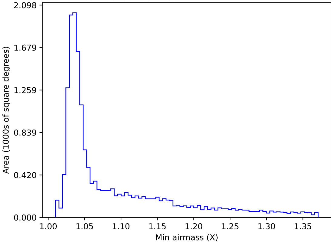
too_elab_r16_d2_giz_v3.4_10yrs WFD g band: Min airmass
