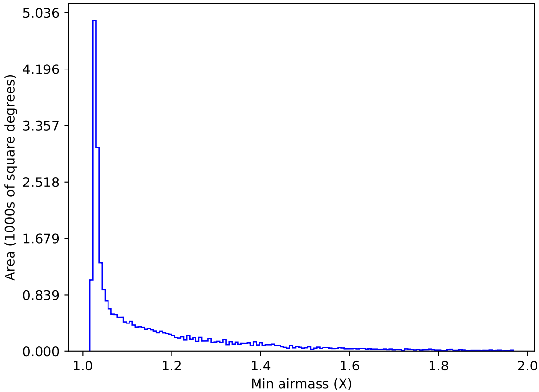
too_elab_r16_d2_giz_v3.4_10yrs All sky z band: Min airmass
