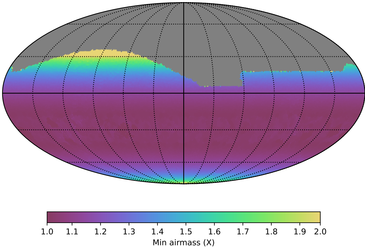
too_elab_r16_d2_giz_v3.4_10yrs All sky g band: Min airmass
