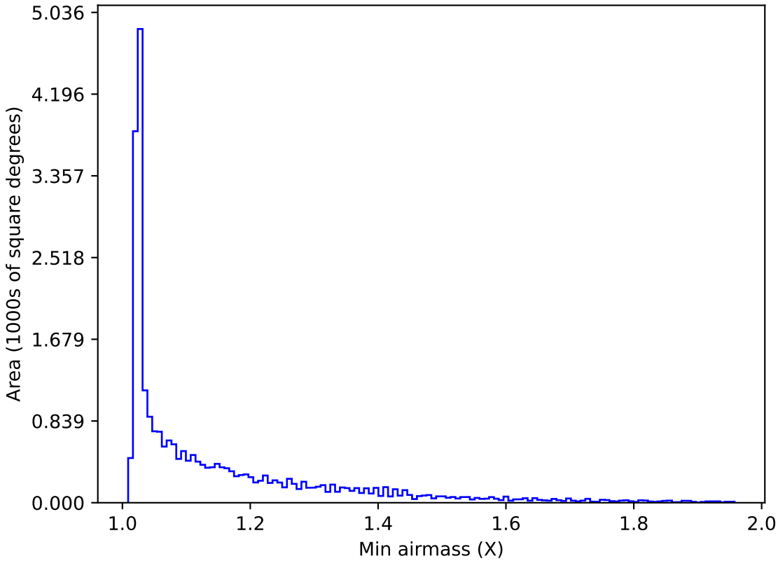
too_elab_r16_d2_giz_v3.4_10yrs All sky all bands: Min airmass
