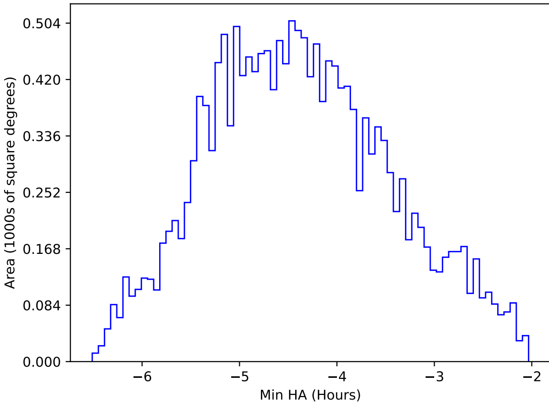
too_elab_r16_d2_giz_v3.4_10yrs WFD z band: Min HA
