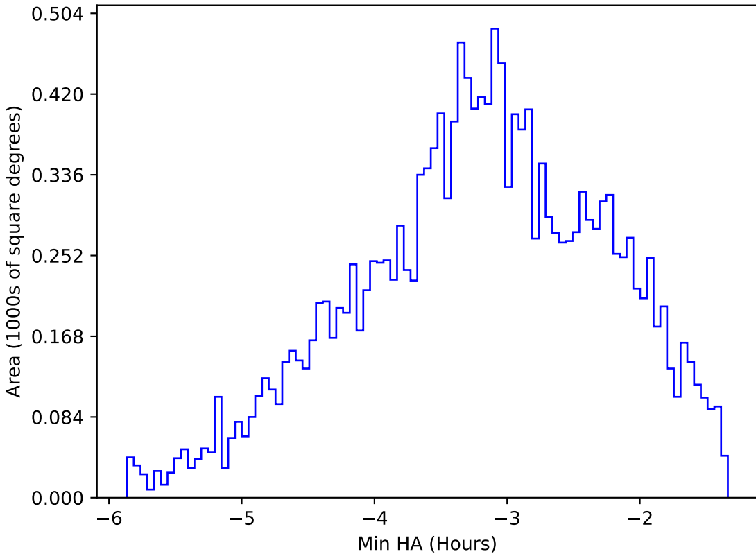
too_elab_r16_d2_giz_v3.4_10yrs WFD u band: Min HA
