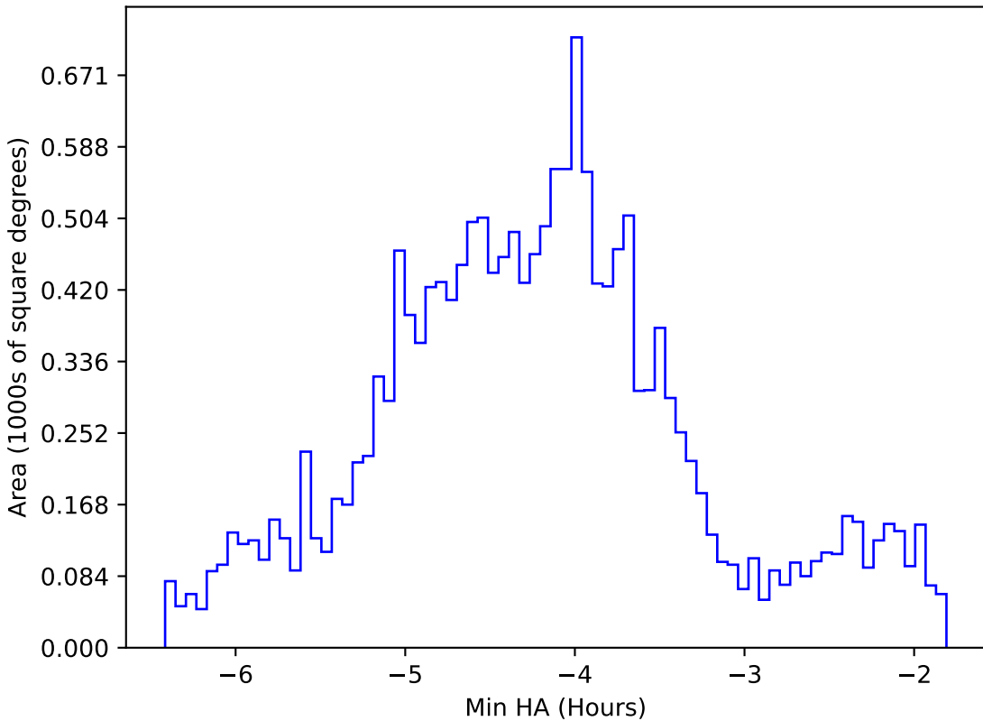
too_elab_r16_d2_giz_v3.4_10yrs WFD g band: Min HA
