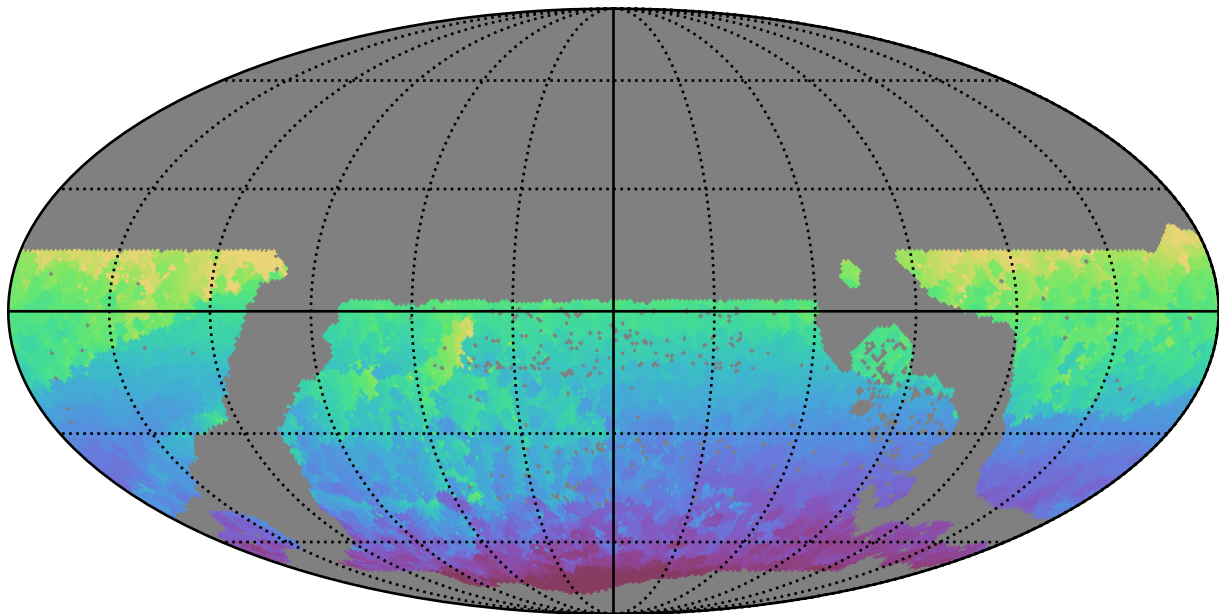
too_elab_r16_d2_giz_v3.4_10yrs WFD all bands: Min HA
