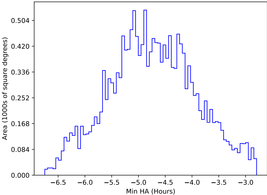
too_elab_r16_d2_giz_v3.4_10yrs WFD all bands: Min HA
