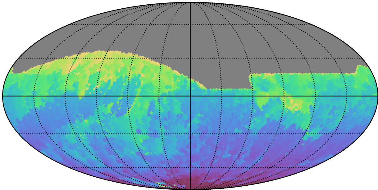
too_elab_r16_d2_giz_v3.4_10yrs All sky z band: Min HA
