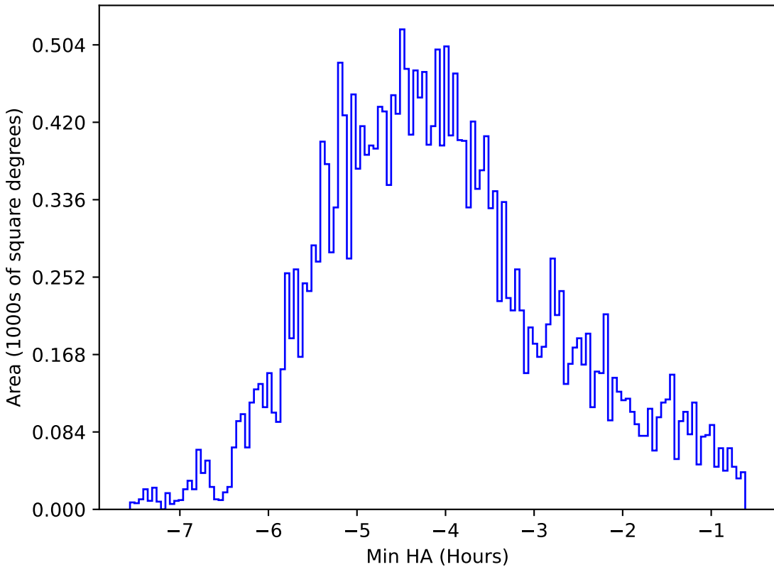
too_elab_r16_d2_giz_v3.4_10yrs All sky z band: Min HA
