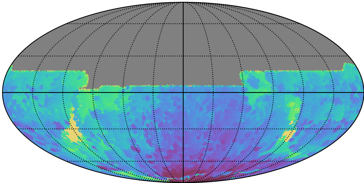
too_elab_r16_d2_giz_v3.4_10yrs All sky y band: Min HA
