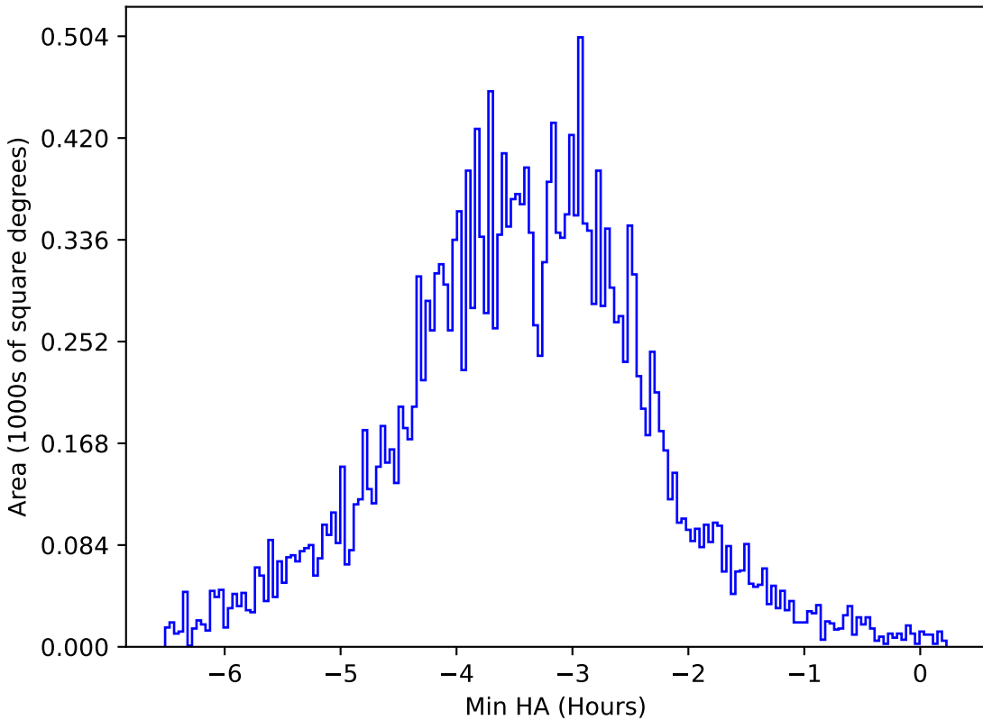
too_elab_r16_d2_giz_v3.4_10yrs All sky y band: Min HA
