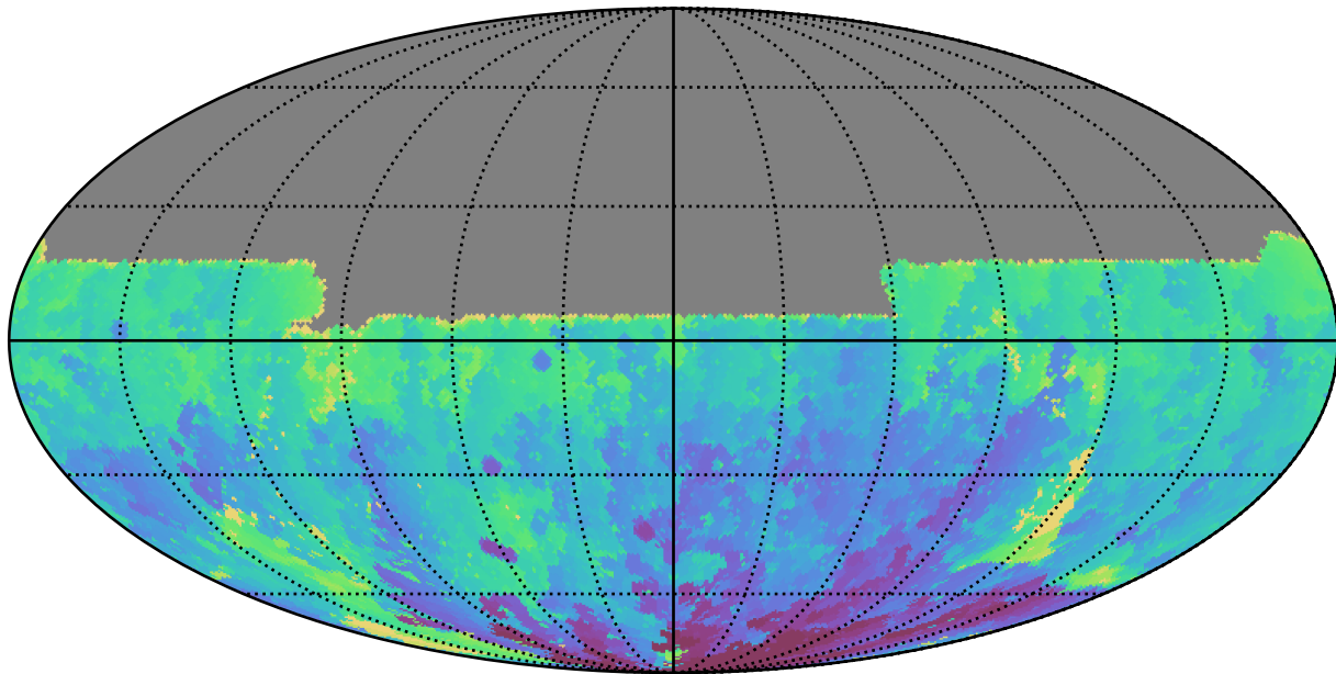
too_elab_r16_d2_giz_v3.4_10yrs All sky u band: Min HA
