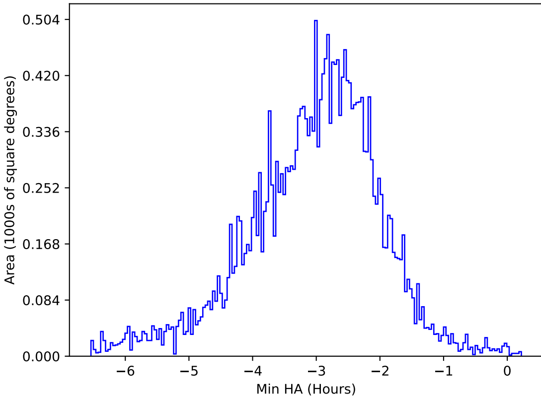
too_elab_r16_d2_giz_v3.4_10yrs All sky u band: Min HA
