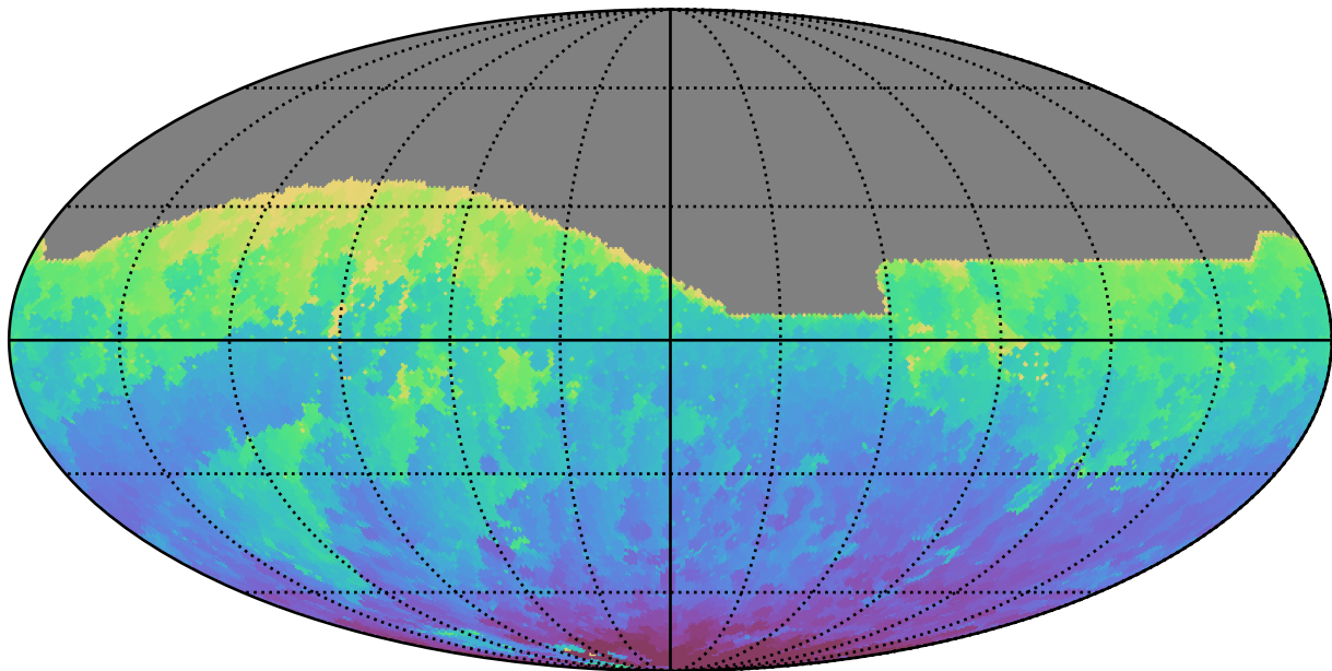
too_elab_r16_d2_giz_v3.4_10yrs All sky i band: Min HA
