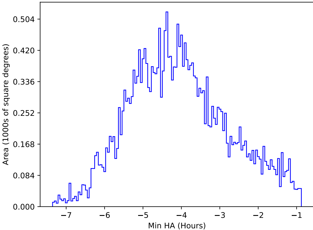
too_elab_r16_d2_giz_v3.4_10yrs All sky i band: Min HA
