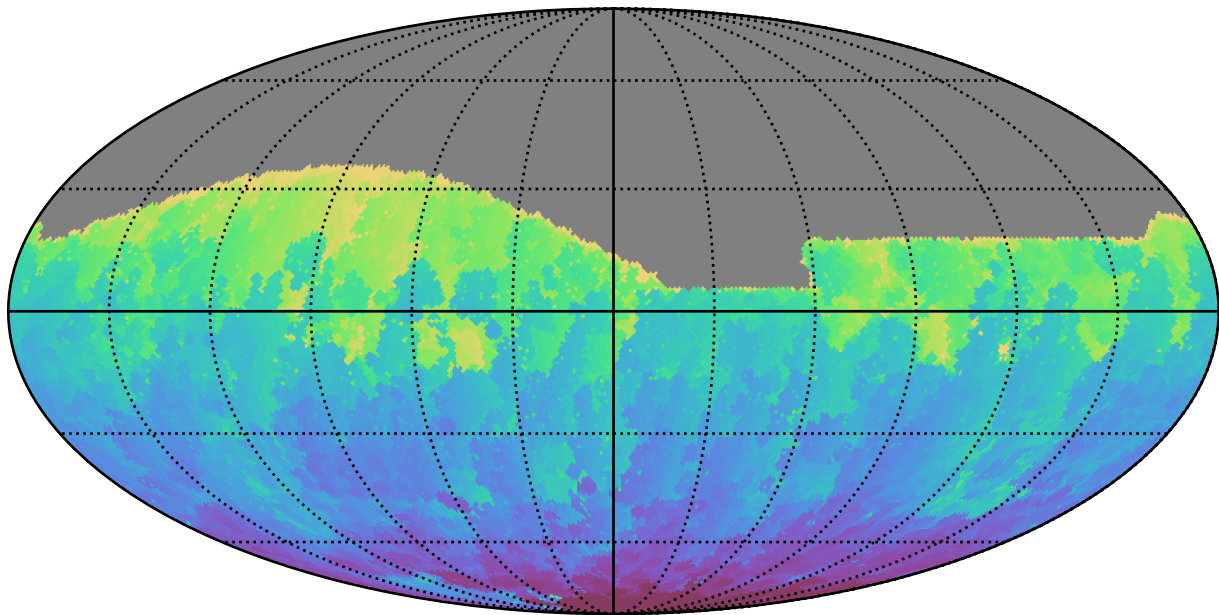
too_elab_r16_d2_giz_v3.4_10yrs All sky g band: Min HA
