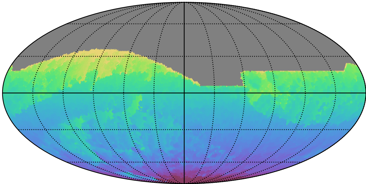
too_elab_r16_d2_giz_v3.4_10yrs All sky all bands: Min HA
