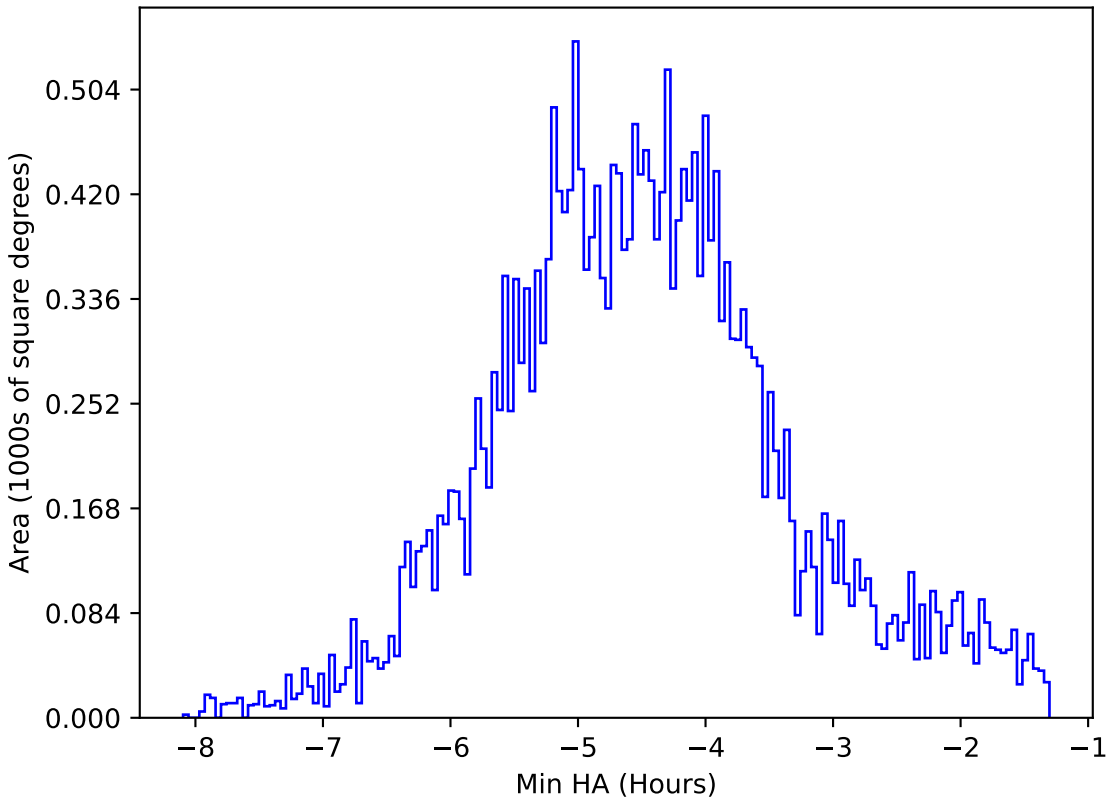
too_elab_r16_d2_giz_v3.4_10yrs All sky all bands: Min HA
