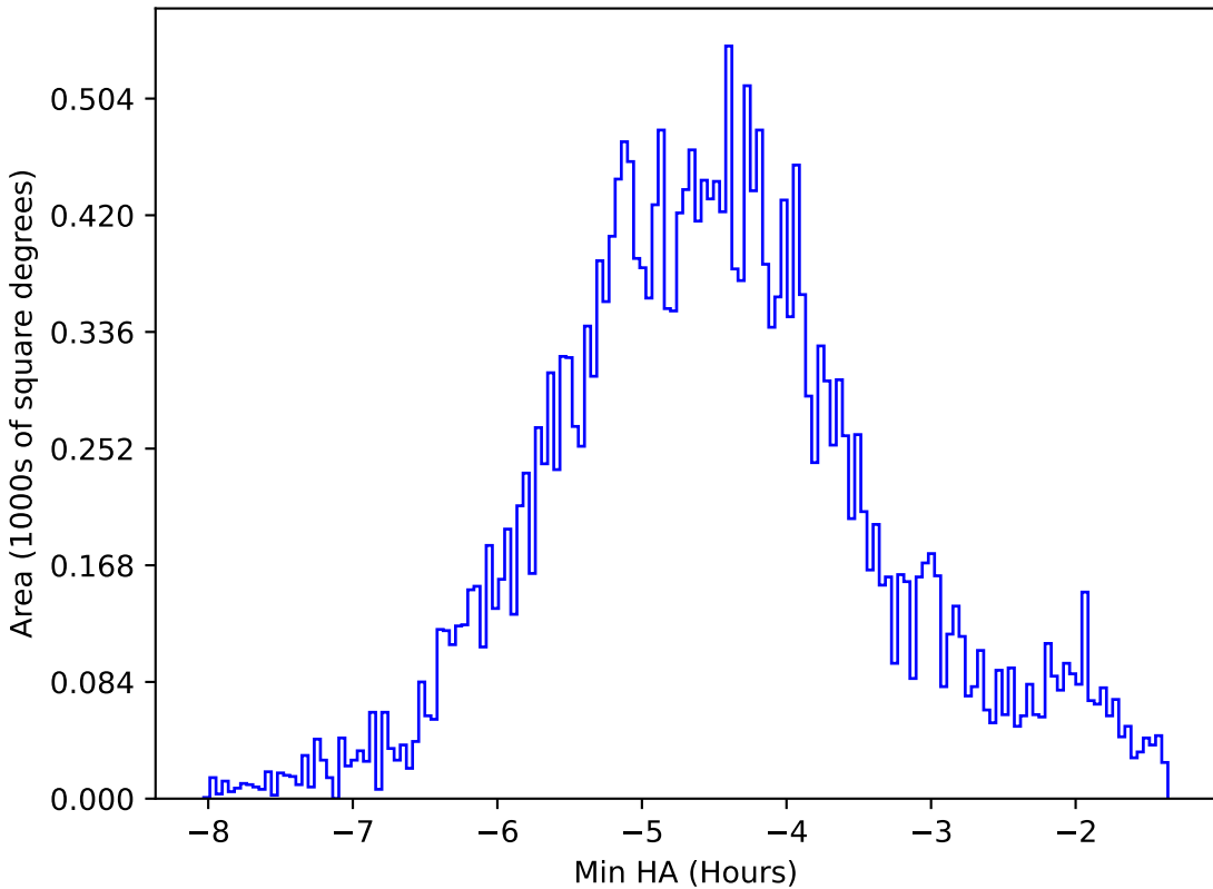
too_elab_r16_d2_giz_v3.4_10yrs All sky all bands: Min HA
