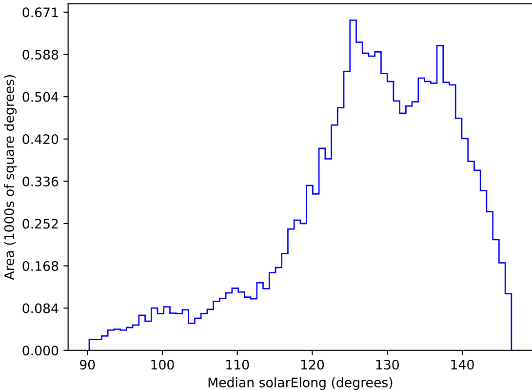
too_elab_r16_d2_giz_v3.4_10yrs WFD z band: Median solarElong
