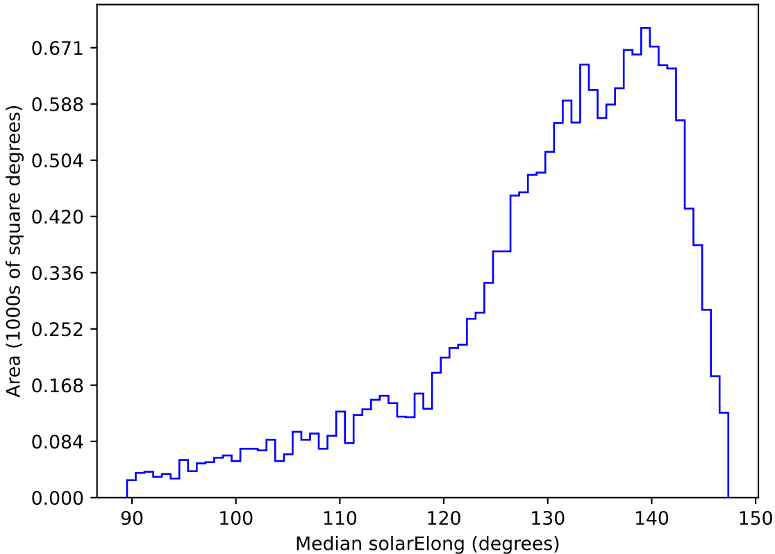
too_elab_r16_d2_giz_v3.4_10yrs WFD y band: Median solarElong
