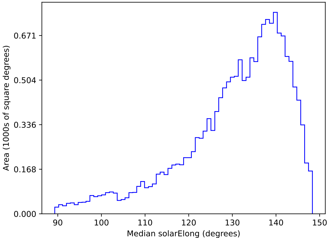
too_elab_r16_d2_giz_v3.4_10yrs WFD r band: Median solarElong
