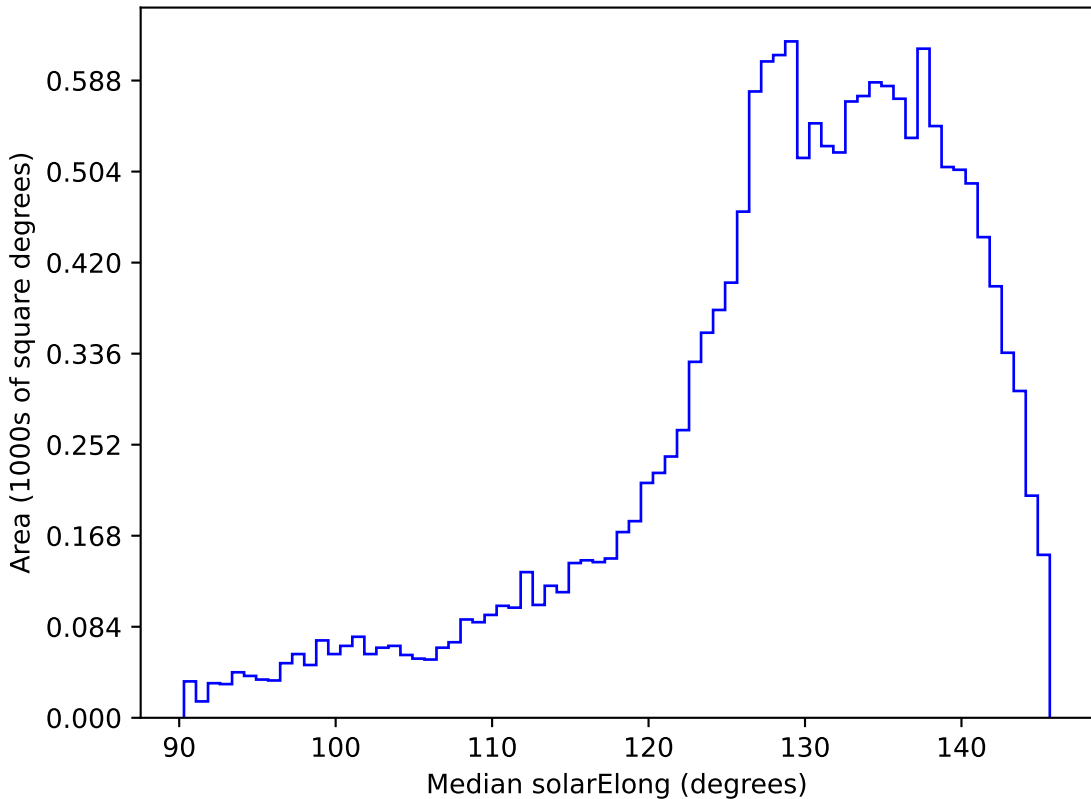
too_elab_r16_d2_giz_v3.4_10yrs WFD i band: Median solarElong
