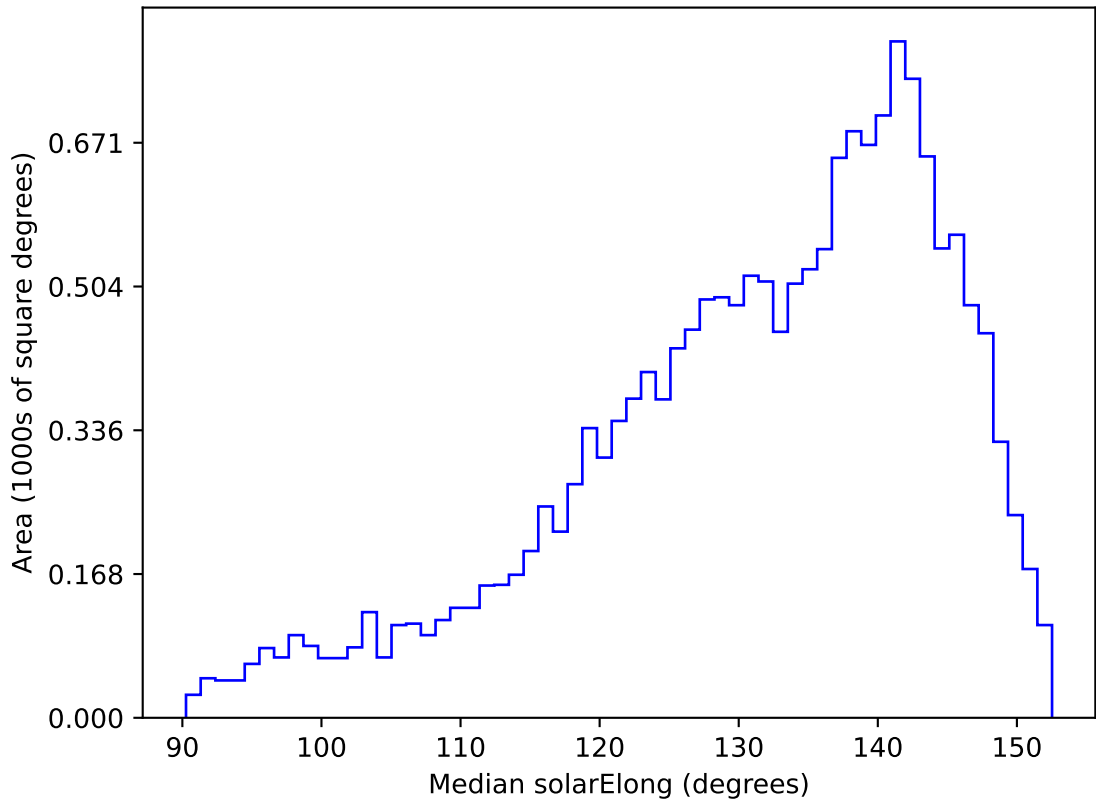
too_elab_r16_d2_giz_v3.4_10yrs WFD g band: Median solarElong
