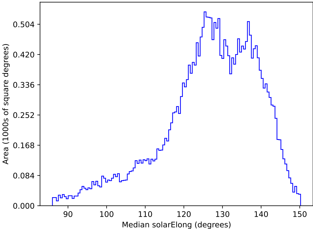
too_elab_r16_d2_giz_v3.4_10yrs All sky z band: Median solarElong
