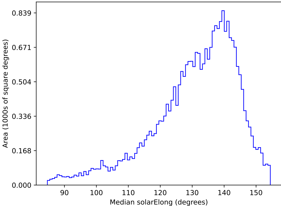
too_elab_r16_d2_giz_v3.4_10yrs All sky r band: Median solarElong
