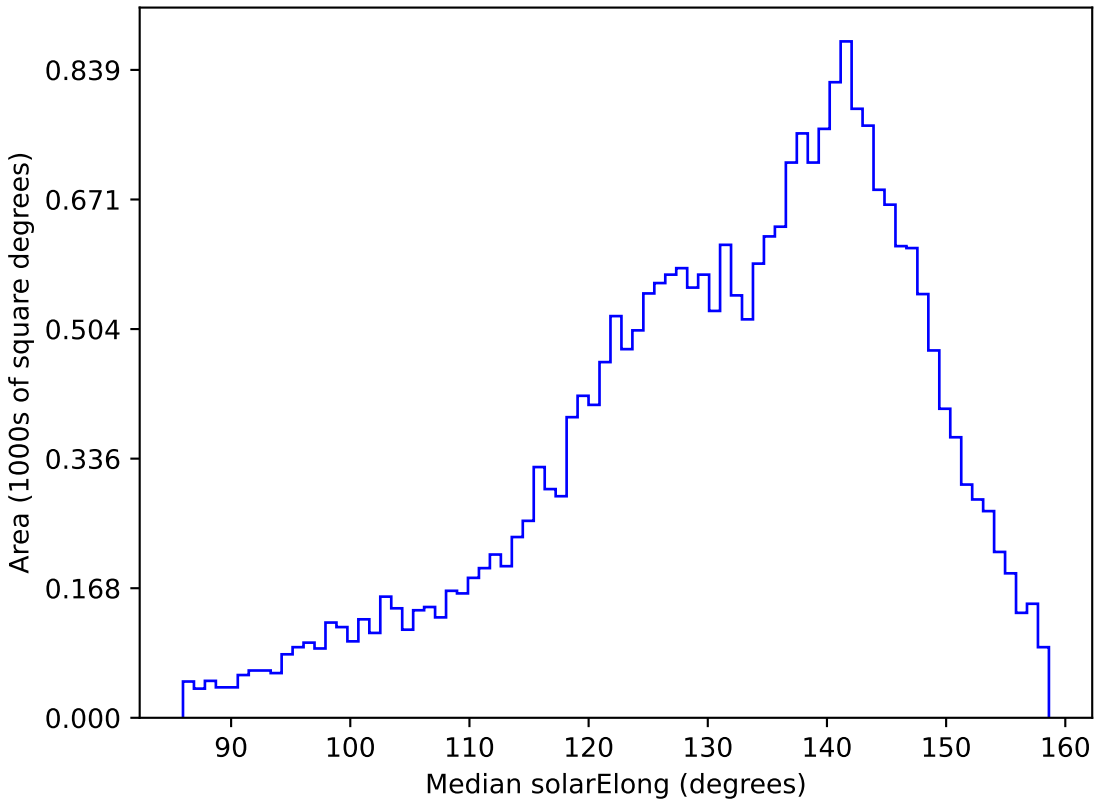
too_elab_r16_d2_giz_v3.4_10yrs All sky g band: Median solarElong
