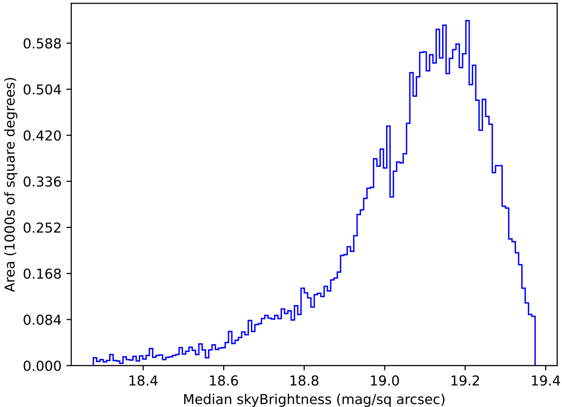
too_elab_r16_d2_giz_v3.4_10yrs Yr 1 z band: Median skyBrightness
