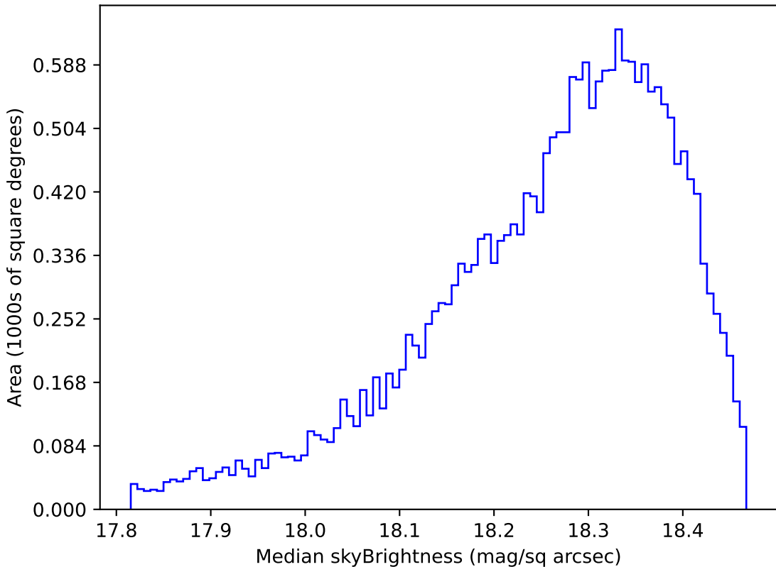
too_elab_r16_d2_giz_v3.4_10yrs Yr 1 y band: Median skyBrightness
