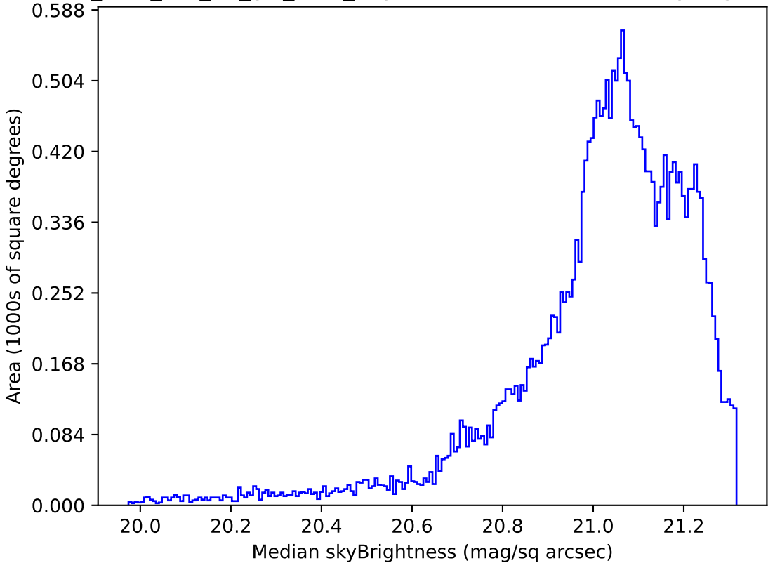
too_elab_r16_d2_giz_v3.4_10yrs Yr 1 r band: Median skyBrightness
