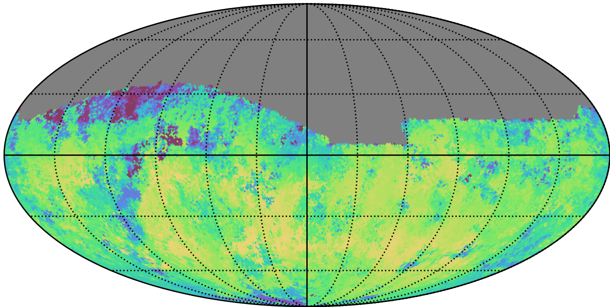
too_elab_r16_d2_giz_v3.4_10yrs Yr 1 i band: Median skyBrightness
