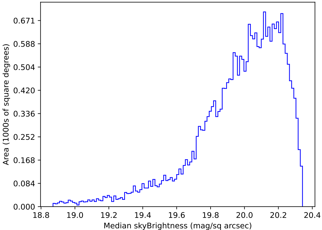
too_elab_r16_d2_giz_v3.4_10yrs Yr 1 i band: Median skyBrightness
