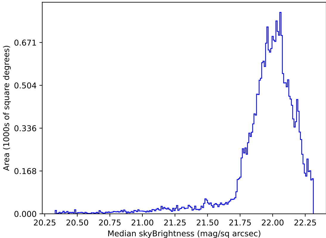
too_elab_r16_d2_giz_v3.4_10yrs Yr 1 g band: Median skyBrightness
