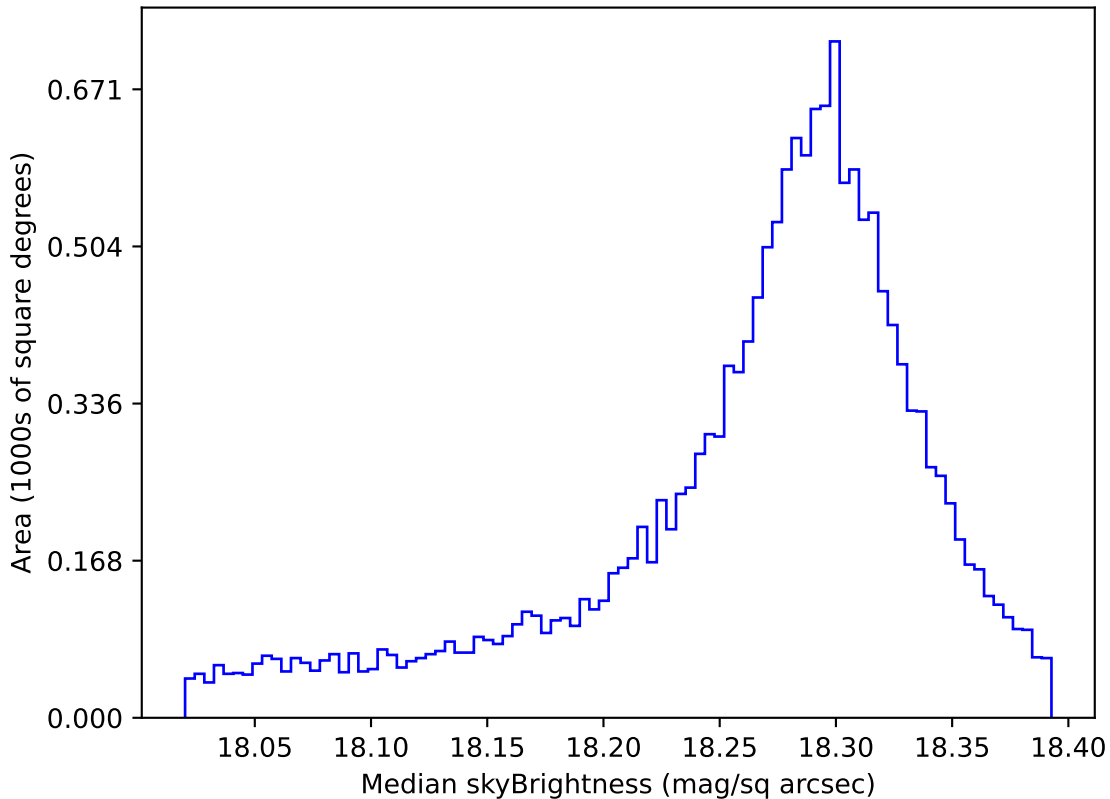
too_elab_r16_d2_giz_v3.4_10yrs WFD y band: Median skyBrightness
