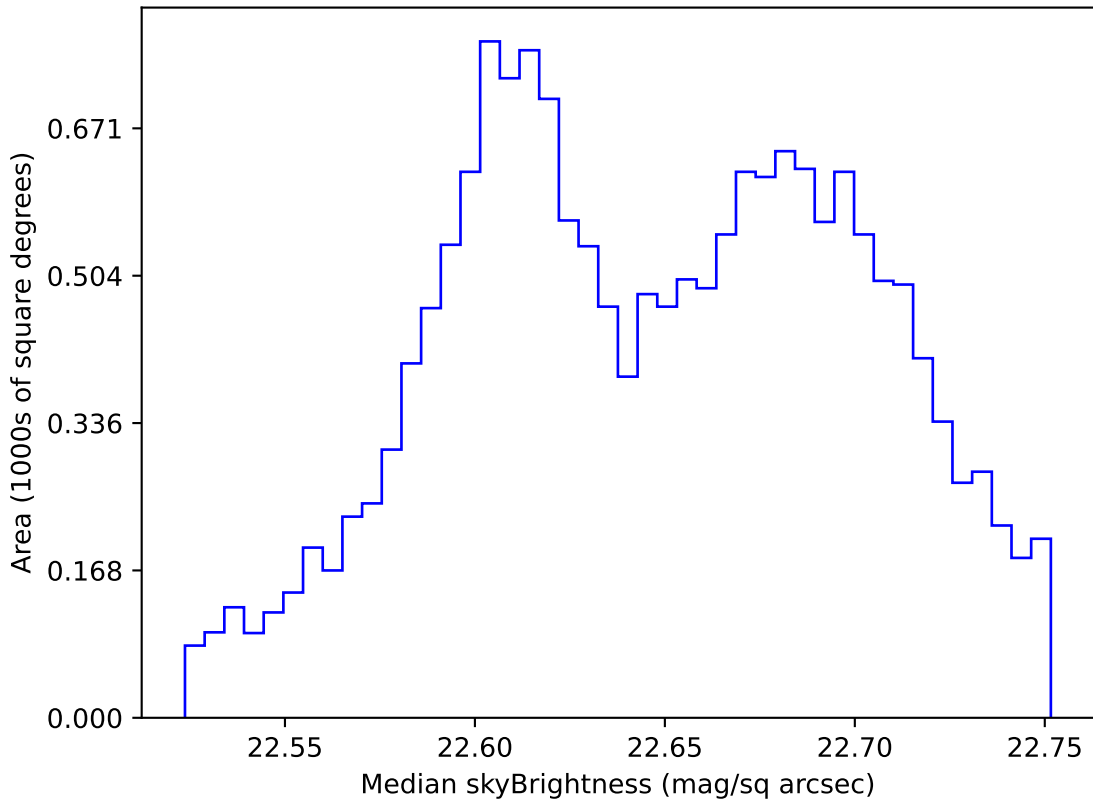
too_elab_r16_d2_giz_v3.4_10yrs WFD u band: Median skyBrightness
