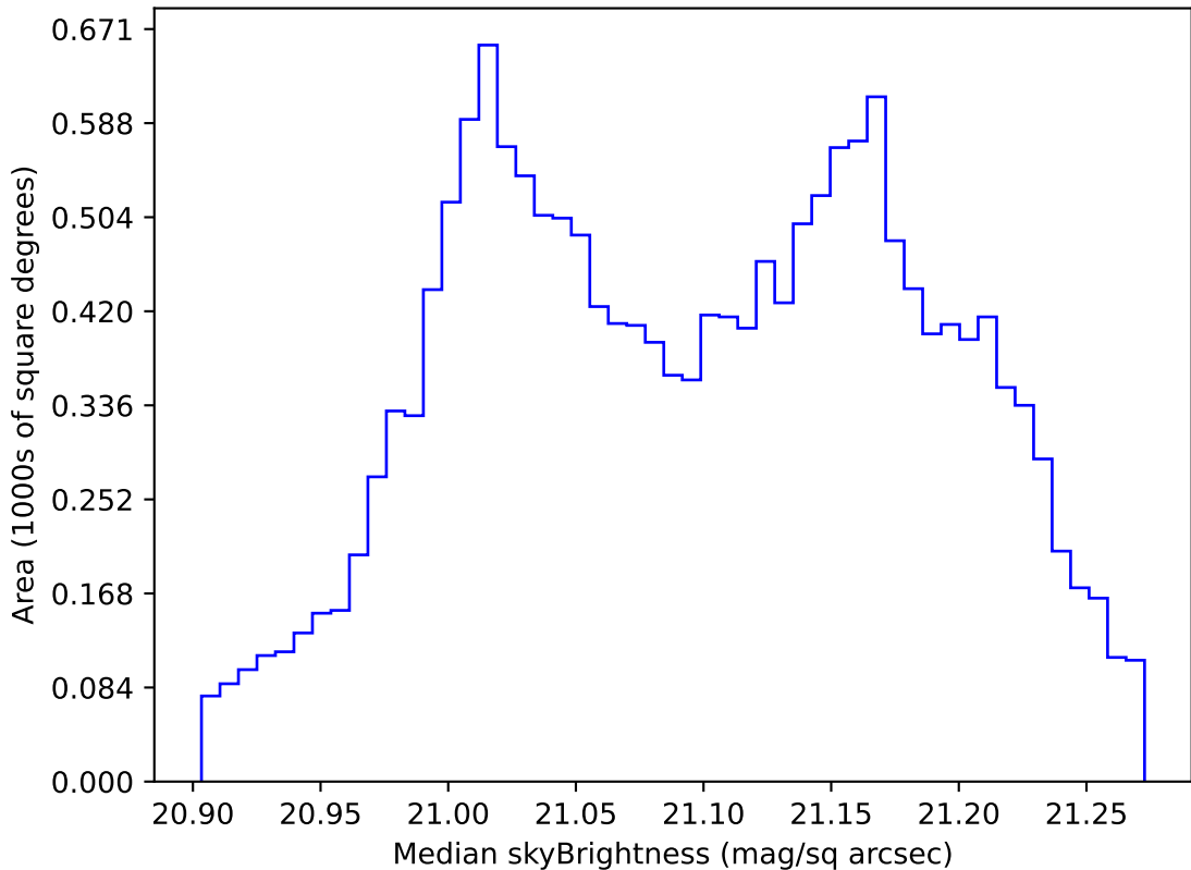
too_elab_r16_d2_giz_v3.4_10yrs WFD r band: Median skyBrightness
