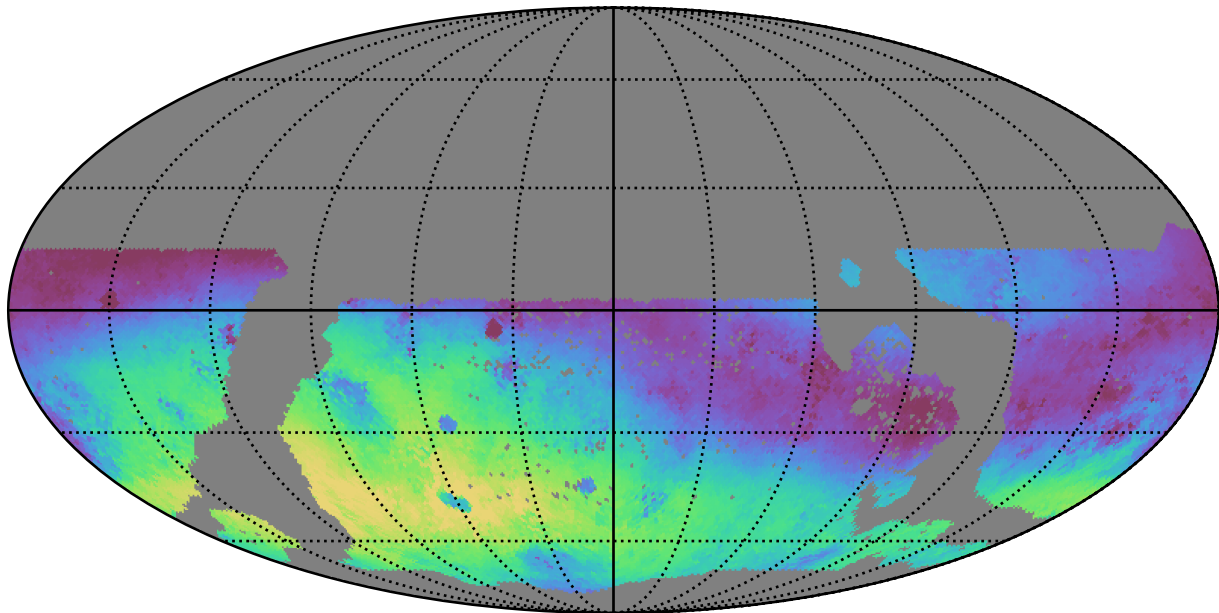
too_elab_r16_d2_giz_v3.4_10yrs WFD g band: Median skyBrightness
