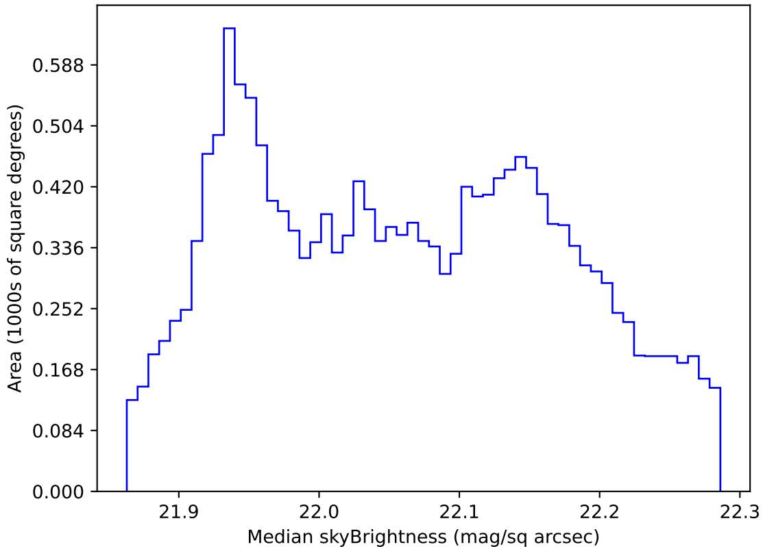
too_elab_r16_d2_giz_v3.4_10yrs WFD g band: Median skyBrightness
