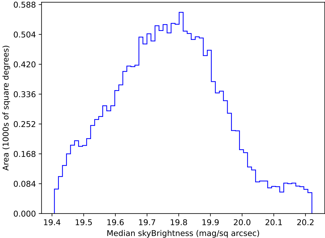
too_elab_r16_d2_giz_v3.4_10yrs WFD all bands: Median skyBrightness
