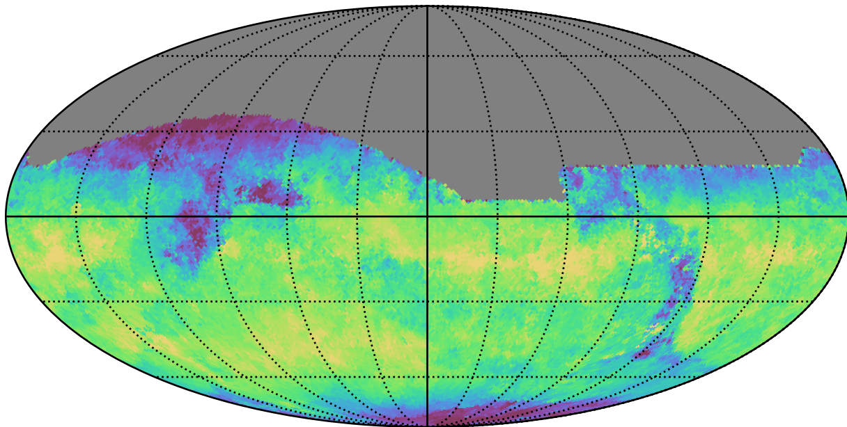
too_elab_r16_d2_giz_v3.4_10yrs All sky z band: Median skyBrightness
