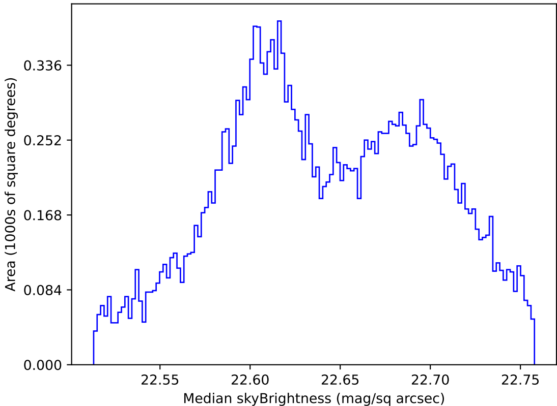
too_elab_r16_d2_giz_v3.4_10yrs All sky u band: Median skyBrightness
