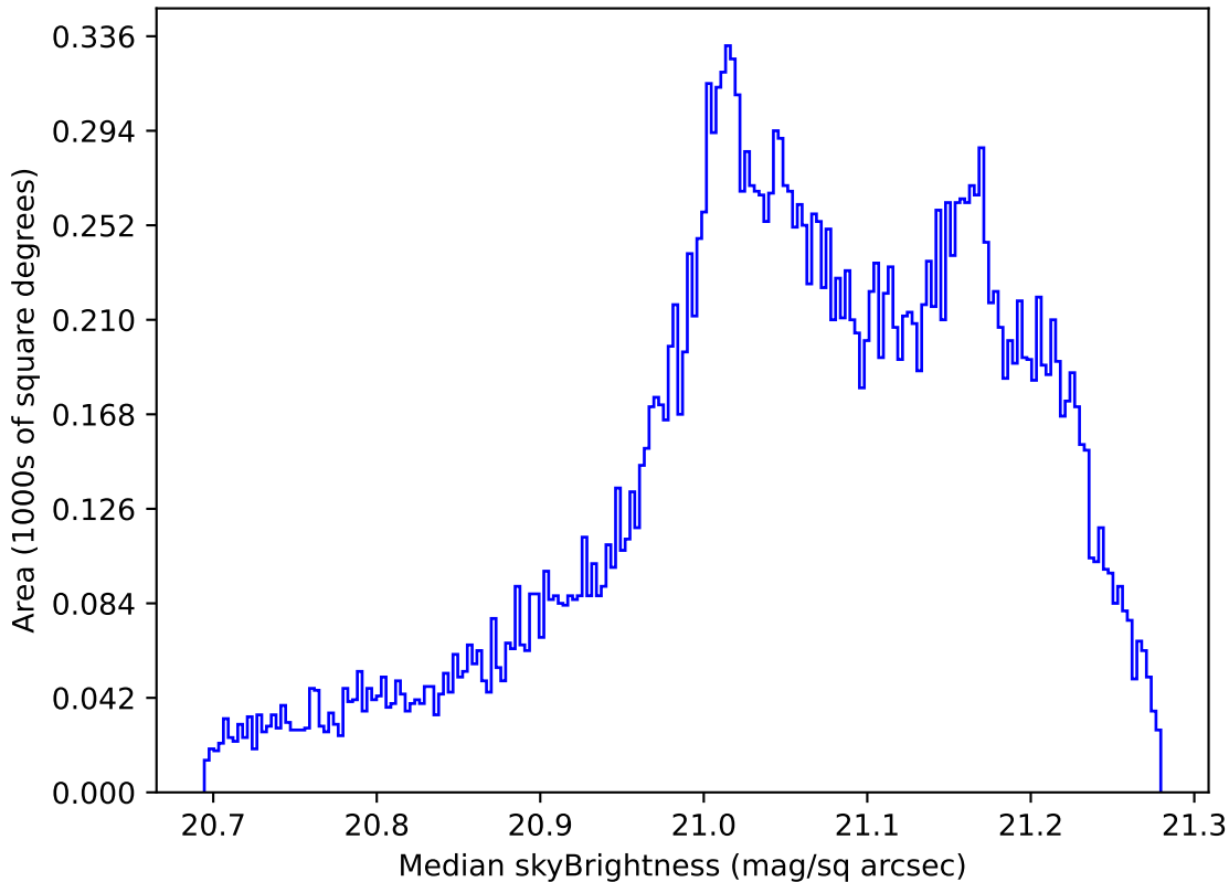
too_elab_r16_d2_giz_v3.4_10yrs All sky r band: Median skyBrightness
