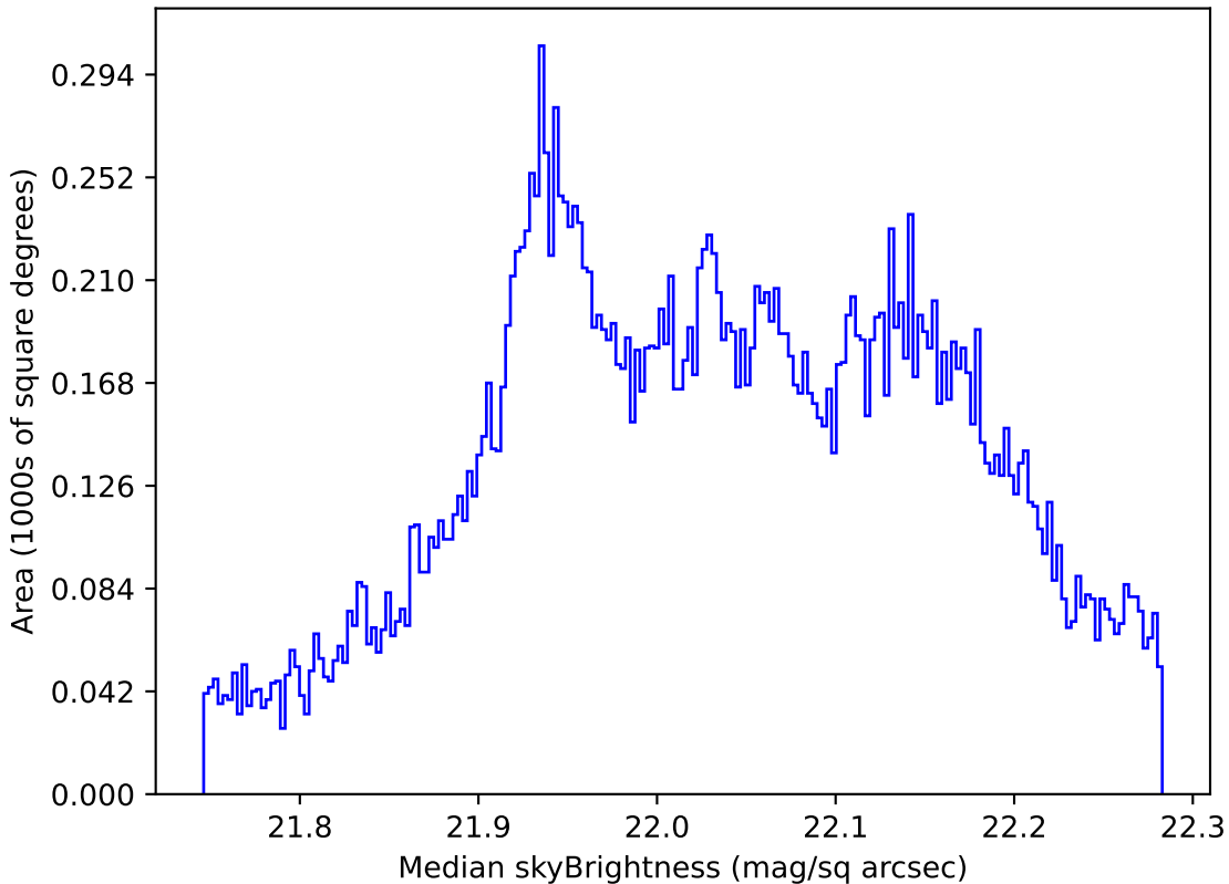
too_elab_r16_d2_giz_v3.4_10yrs All sky g band: Median skyBrightness
