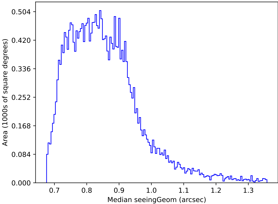
too_elab_r16_d2_giz_v3.4_10yrs Yr 1 z band: Median seeingGeom
