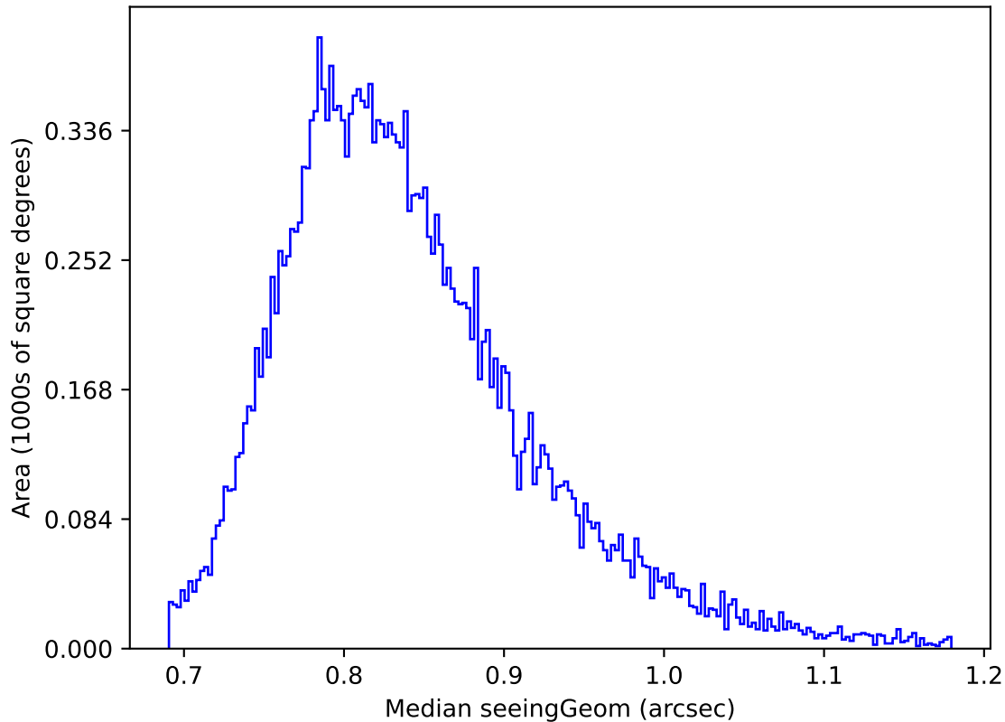
too_elab_r16_d2_giz_v3.4_10yrs Yr 1 y band: Median seeingGeom
