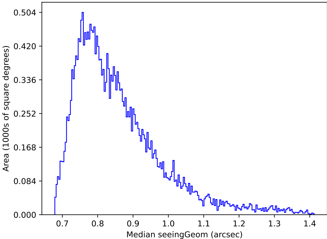
too_elab_r16_d2_giz_v3.4_10yrs Yr 1 r band: Median seeingGeom
