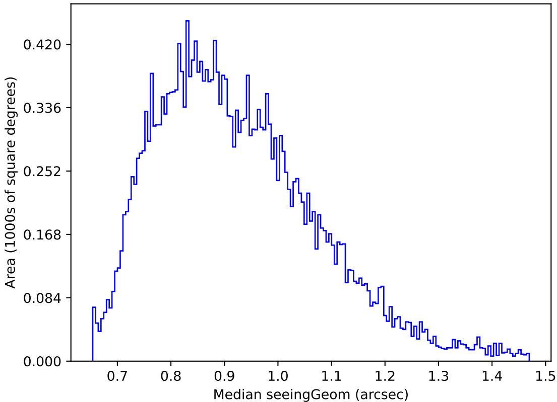
too_elab_r16_d2_giz_v3.4_10yrs Yr 1 g band: Median seeingGeom
